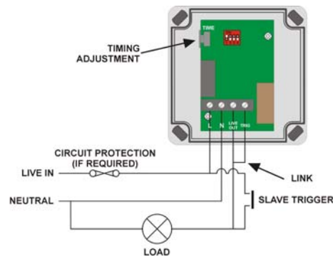
Diagram 2 Wiring for three wire switching circuits
