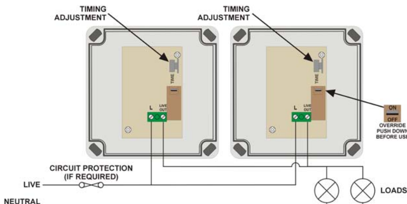
Diagram 2 Multiple switch locations
