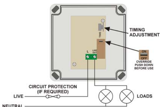
Diagram 1 Conventional wiring
